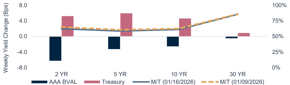
FIGURE 1: MUNIS OUTPERFORM 2
